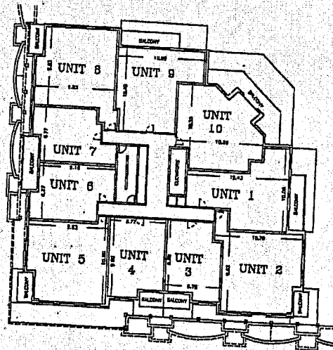
UNITS 1 to 10 (inclusive), LEVELS 5 to 14 (inclusive) (NOT TO SCALE)
