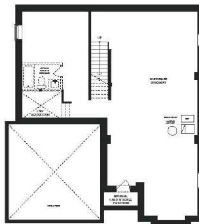
Basement ELEVATION 'A'
